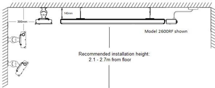
Diagram 2: Mounting options and minimum distances to objects.
